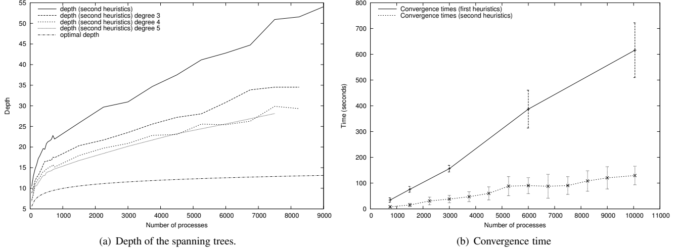
Figure 1. Scalability of the spanning tree algorithm.
